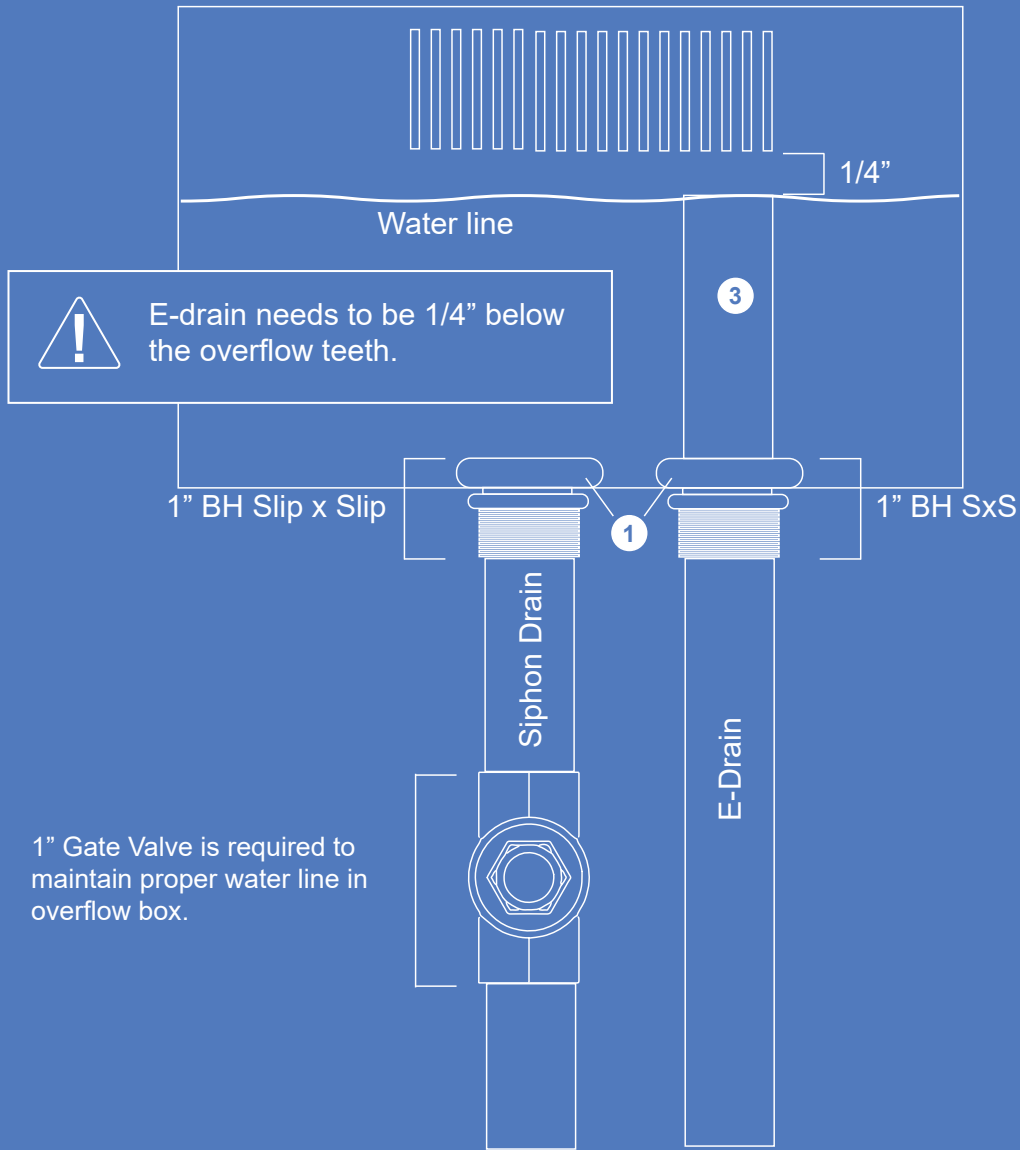
EXTERNAL OVERFLOW BOX [REAR VIEW]
